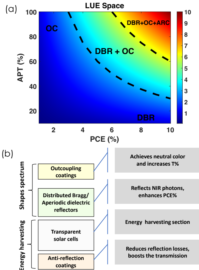
Figure: (a) Light utilization efficiency (LUE) space illustrating the competition between average photopic transmittance (APT) and power conversion efficiency (PCE) encountered in the design of ST-OPVs. (b) Design schematics of various sections of the ST-OPV.
