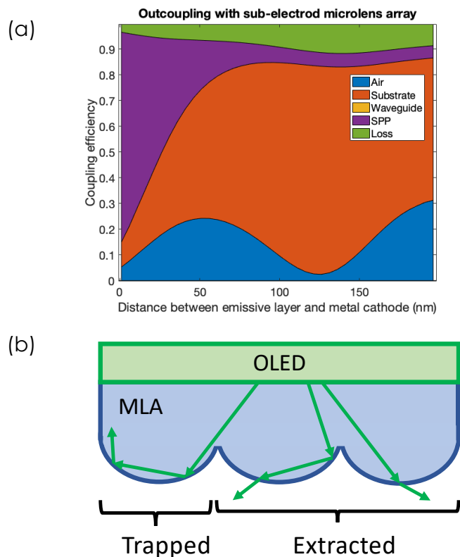
Figure: (a) Fraction of light coupled into the substrate mode of a green phosphorescent OLED. (b) Schematic of a typical microlens array outcoupling structure. Light is trapped due to the index mismatch between the microlens array and air.
