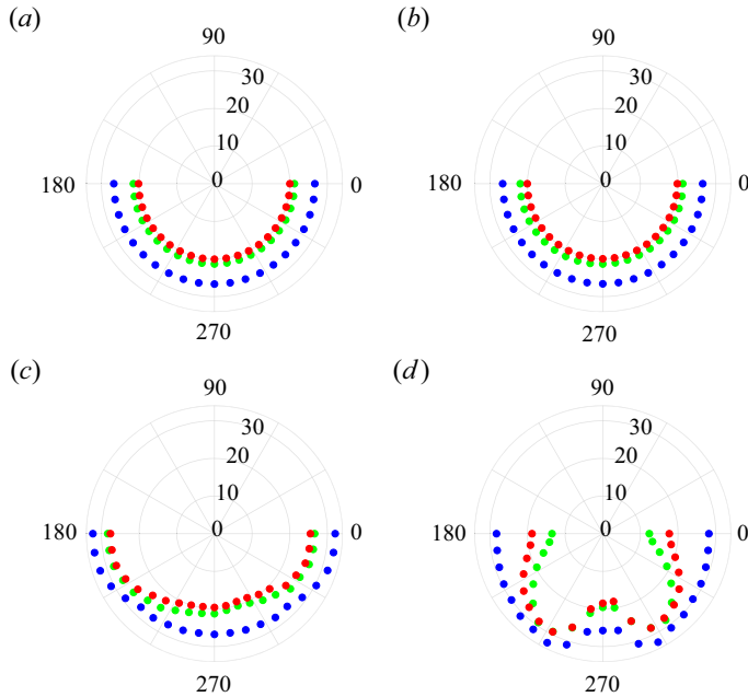
Figure 25. Acoustic radiation pattern ( P_{pattern} = 20 \log_{10}(P_{RMS}^a / 20 \times 10^{-6}) , where P_{RMS}^a is the r.m.s. acoustic pressure) at r = 30\delta for synthetic rubber plates at Re_\tau = 180 : (a–d) \gamma_o^{(1)} , 10\gamma_o^{(1)} , 100\gamma_o^{(1)} and 300\gamma_o^{(1)} . Blue, green, red circles: SSSS, CCCC, CCCF.
