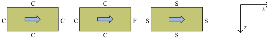
Figure 2. Plate BCs. Arrow denotes the direction of mean flow.
