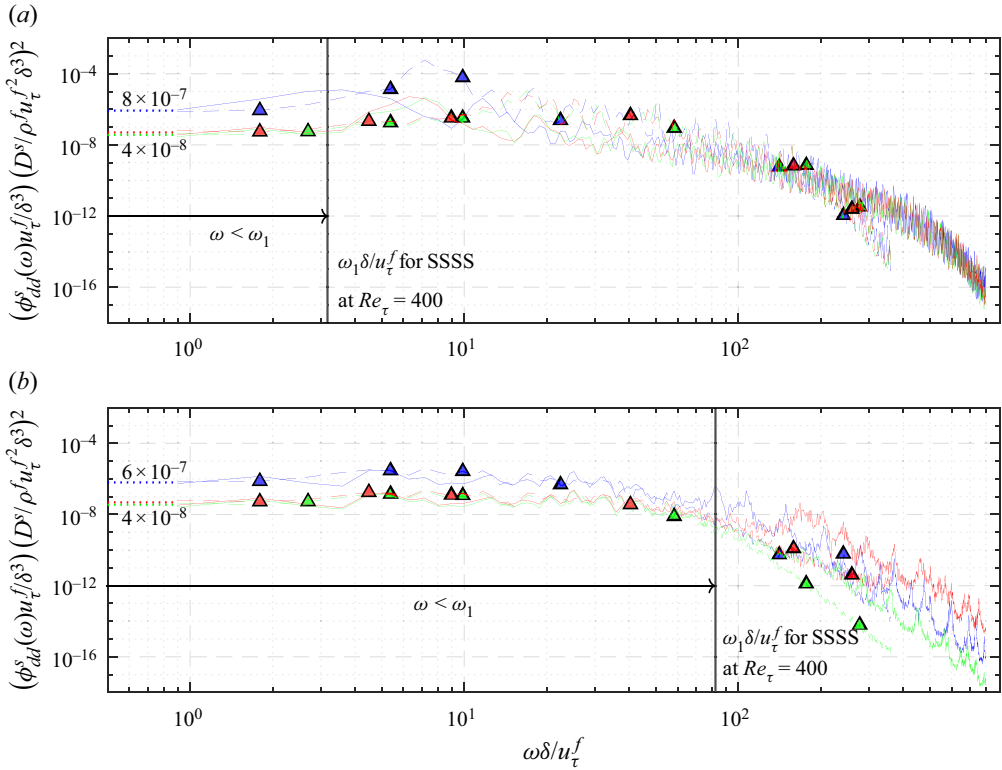
Figure 18. The DNS-based (\phi_{dd}^s(\omega) u_\tau^f / \delta^3) (D^s / \rho^f u_\tau^f{}^2 \delta^3)^2 versus \omega \delta / u_\tau^f for (a) synthetic rubber and (b) stainless steel plates. Blue, green, red triangles: SSSS, CCCC, CCCF at Re_\tau = 180 ; blue, green, red lines: SSSS, CCCC, CCCF at Re_\tau = 400 . Dotted lines of the same colour show the y intercept of the spectrum for each BC.
