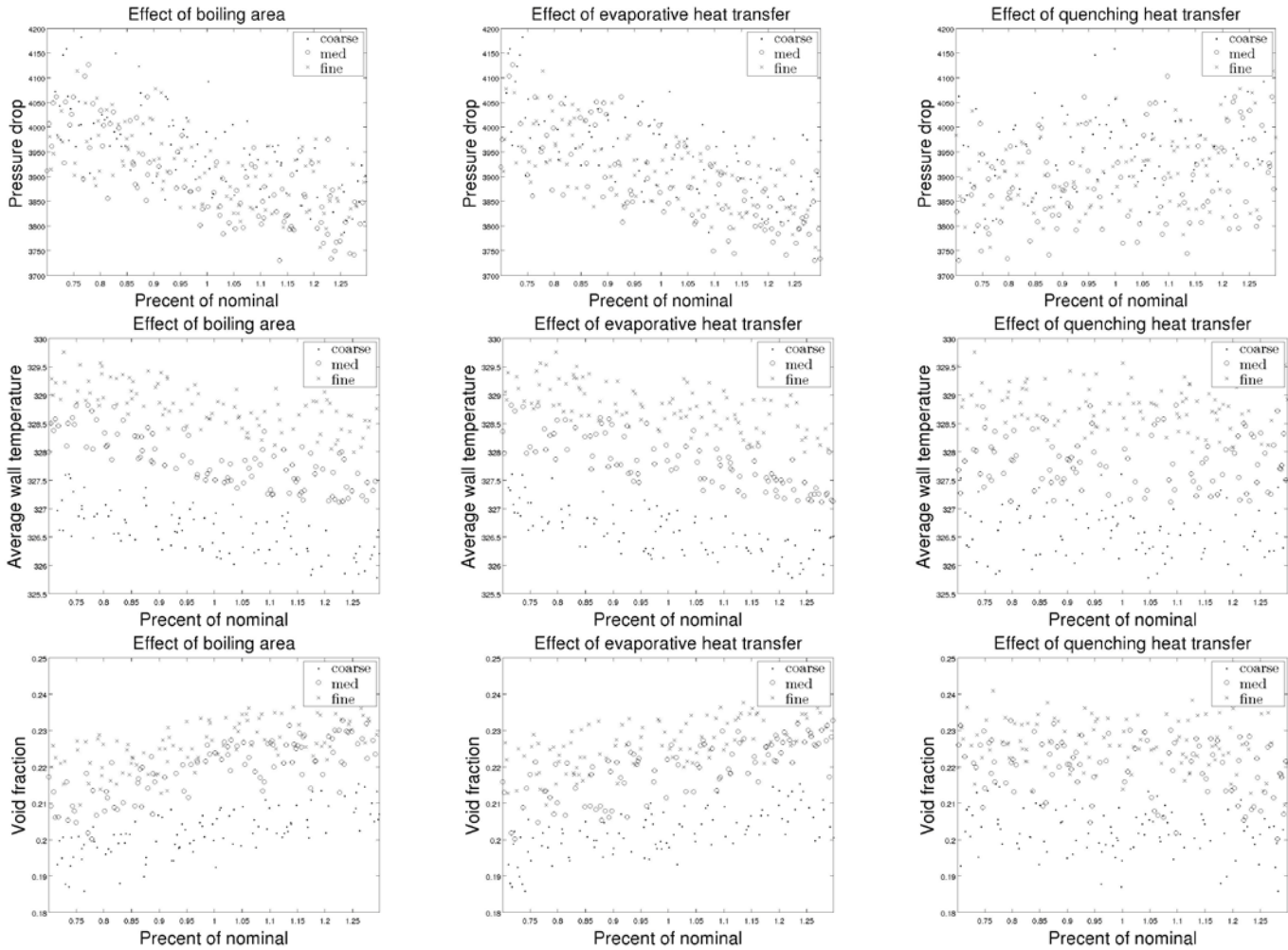
Figure 5. Sensitivity of outputs to boiling area, evaporative heat transfer, and quenching heat transfer
