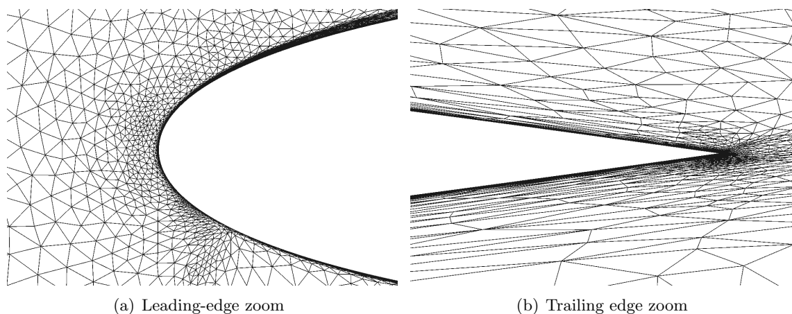
Figure 16. NACA 0012, \alpha = 10^\circ : Close-up of the leading and trailing edges for the 12 th adapted mesh in a drag refinement sequence.
