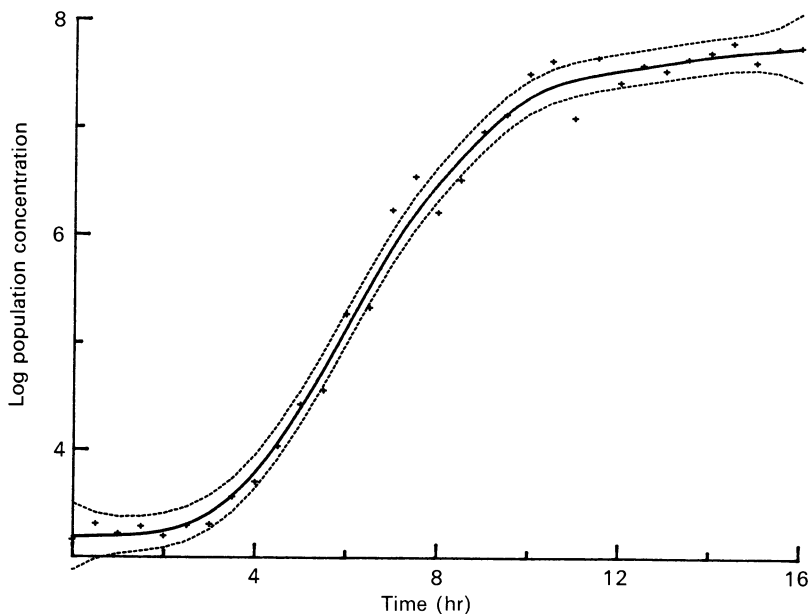
Fig. 8. Microbiological data, with estimated growth curve and probability intervals.
