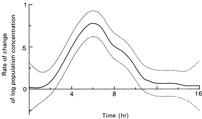
Fig. 9. Estimated growth rate for microbiological data, with probability intervals.
