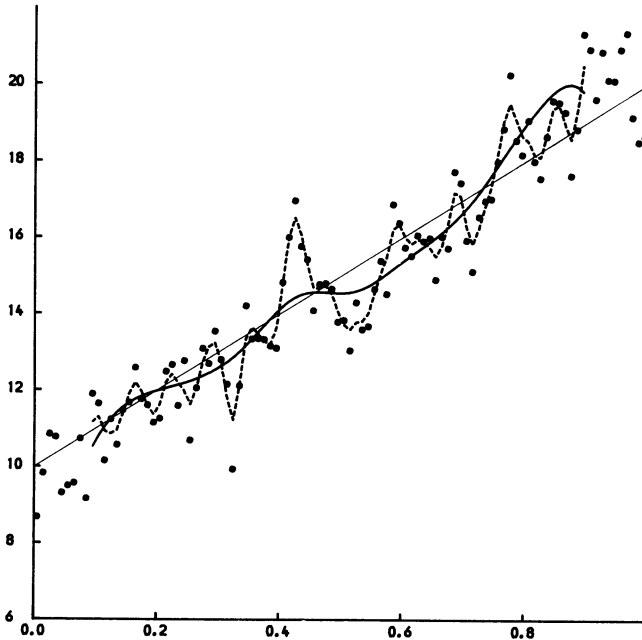
Fig. (D3). Simulation of linear g(t) with autoregressive errors, \rho = 0.75 . Fine solid line shows g(t) = 10(1 + t) . \bullet data; - - - \hat{g}(t) assuming \rho = 0 ; — \hat{g}(t) assuming \rho = 0.75 .
