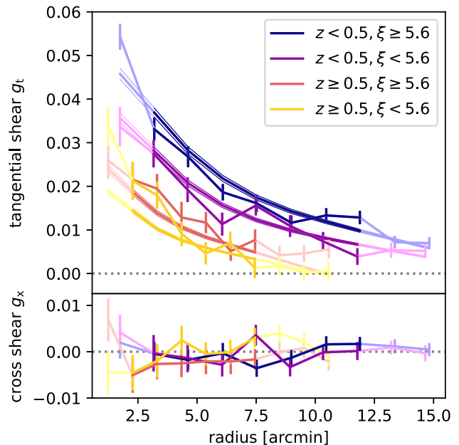
FIG. 2. Stacked DES Y3 lensing shear profiles. Upper panel: tangential shear, along with the mean model prediction from an analysis of the cluster abundance and cluster lensing. The likelihood analysis is performed on a cluster-by-cluster basis, the stacks are only shown for validation purposes. The dark shading shows the radial ranges used in the analysis, light shaded data points outside that range are only shown for reference. For the 26 data points included in the analysis, we measure a signal-to-noise ratio of 32.2 and we obtain a reduced \chi^2_{\text{red}} = 1.48 between the data and the model. Lower panel: within the radial ranges used in the analysis, the cross shear is consistent with null with \chi^2_{\text{red}} = 0.90 .
