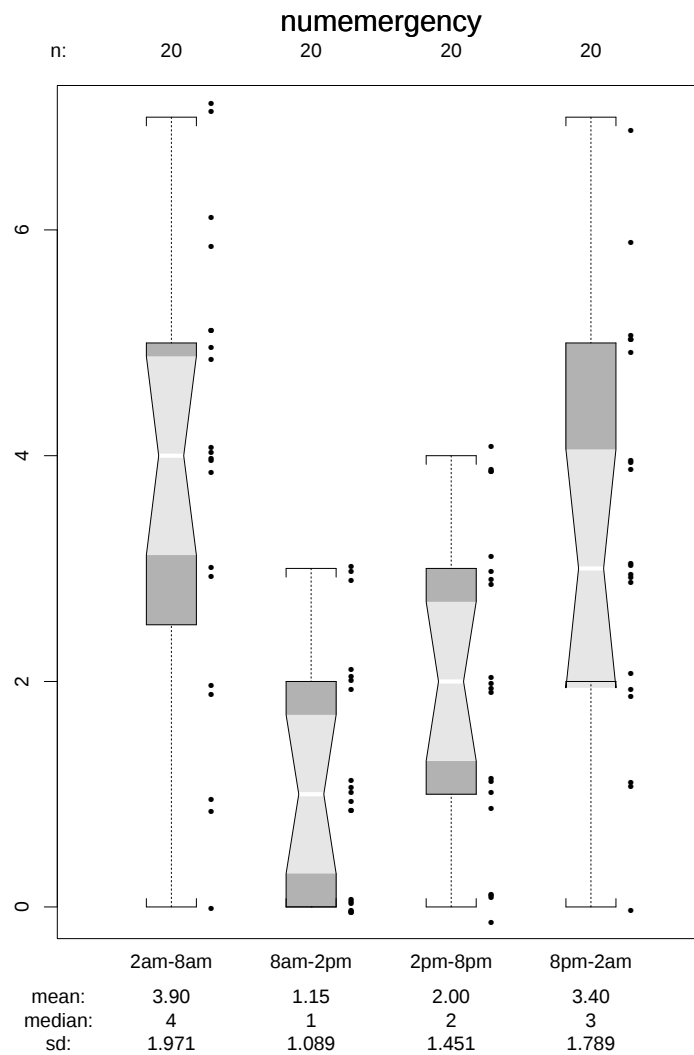
Figure 2-8: Raw helicopter data. Transformation doesn't seem to be needed here. This is a different form of the boxplot, called a notched boxplot, where the light gray notch depicts plus/minus one standard error around the median and the dark gray still represents the usual middle 50%. The standard error around the median is typically defined as 1.5 \cdot \text{IQR} / n .
