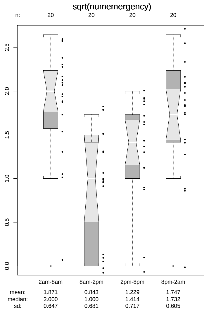
Figure 2-9: Square root of the helicopter data. The spread and level plot suggests that if a transformation is needed, then it might be the square root given that we limit ourselves to the “power family”. It isn’t clear that the transformed boxplot is any better than the original. So, we’d opt for not performing a transformation for these data.
