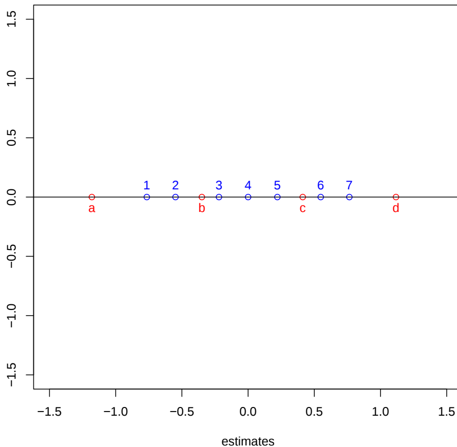
Unfolding in the smacof package
