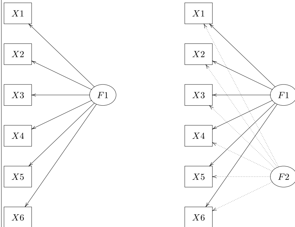
Figure 11-9: LEFT: Representation of a single factor ( F1 ) and its corresponding observed variables ( X1 to X6 ). RIGHT: Representation of two factors ( F1 and F2 ) and corresponding observed variables ( X1 to X6 ).
