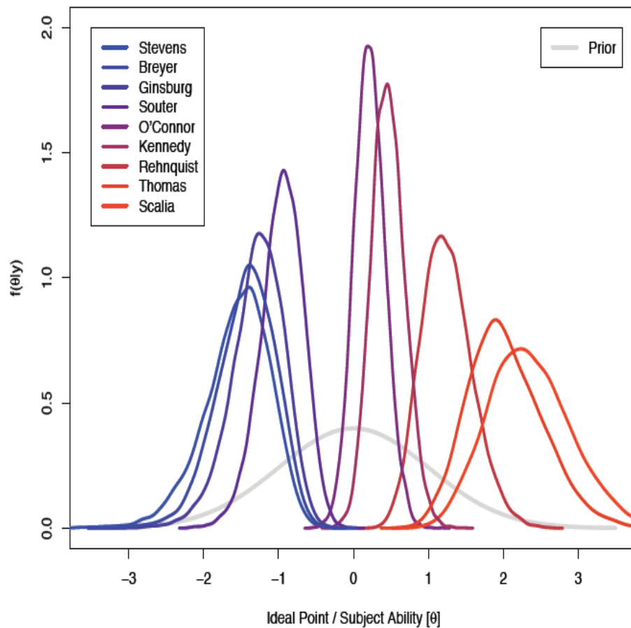
Figure 11-3: 2000 Supreme Court Cases, Bayesian Analysis with Ideal Distributions (MCMCpack tutorial).
