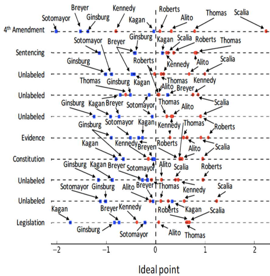
Figure 11-2: 2000 Supreme Court Cases (Islam et al).
