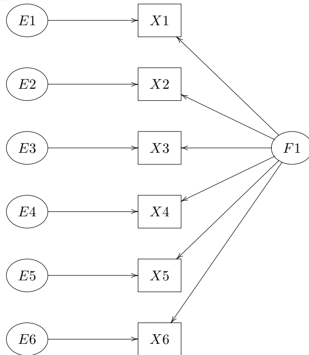
Figure 11-12: Representation of a single factor ( F1 ), its corresponding observed variables ( X1 to X6 ), and the errors.
