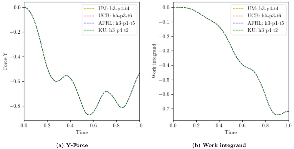
Figure 11: Cylinder Motion-1 Time Histories (finest space-time resolution data-sets from each participant)
