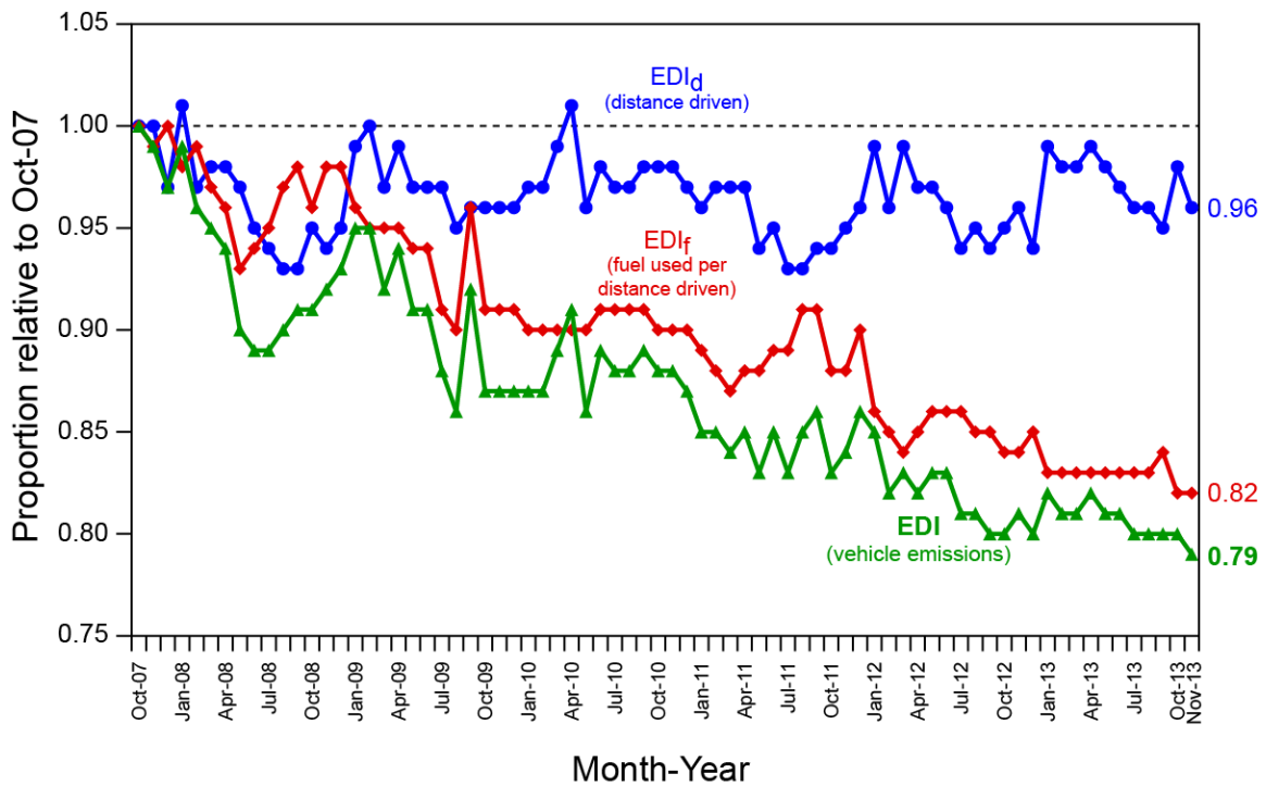
Figure 1. University of Michigan Eco-Driving Index (EDI) and the two sub-indices ( EDI_d and EDI_f ) for October 2007 through November 2013.
