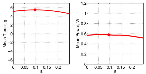
(f) Feathering axis offset
