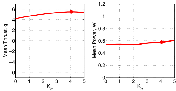
(e) Shape parameter for pitch motion
