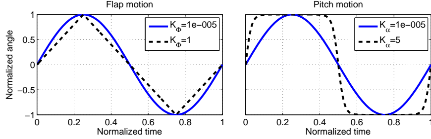
Figure 5. Variation of flap and pitch kinematic patterns with shape parameters
