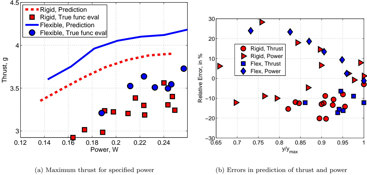
Figure 10. Constrained optimization of rigid and flexible wings
