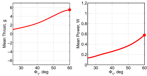
(a) Flap amplitude
