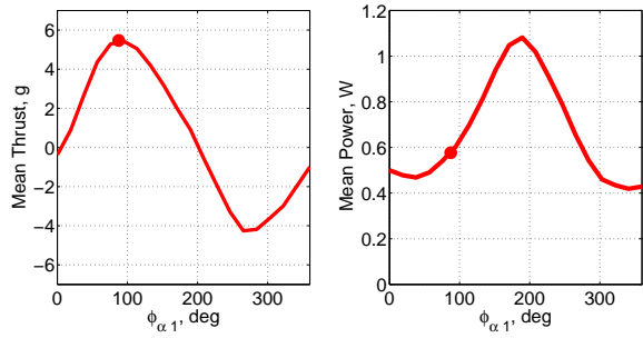
(c) Phase angle
