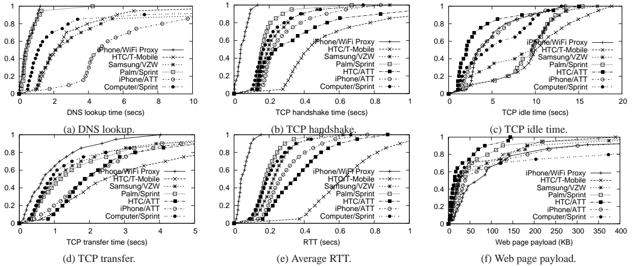
Fig. 5. Breakdown of Web transaction performance: (a)-(d), RTT and Web page payload distribution.
