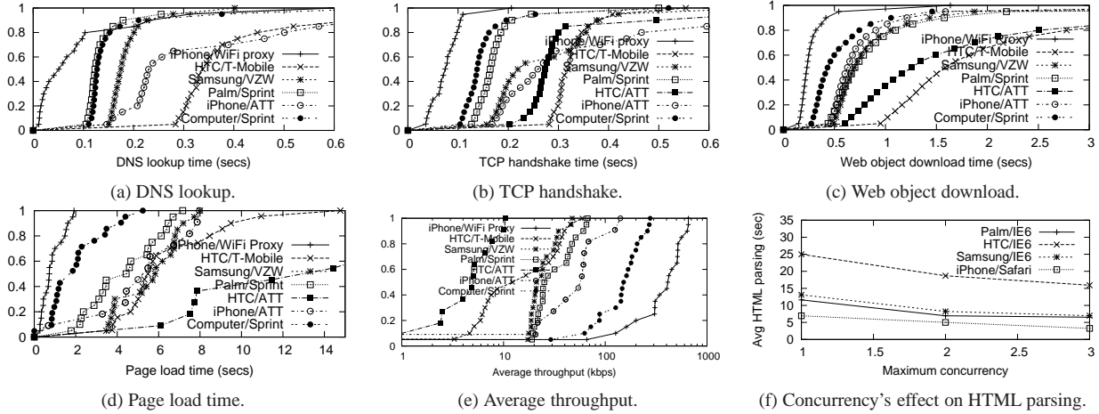
Fig. 8. Controlled experiments for Web transaction breakdown.
