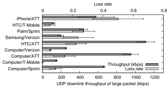
Fig. 1. UDP results across platforms and carriers .
