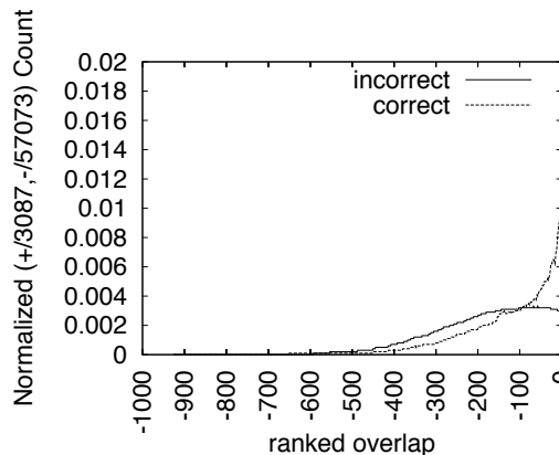
Figure 5: \Pr(\text{rank}=x | [\text{in}] \text{correct}) for TREC-8
